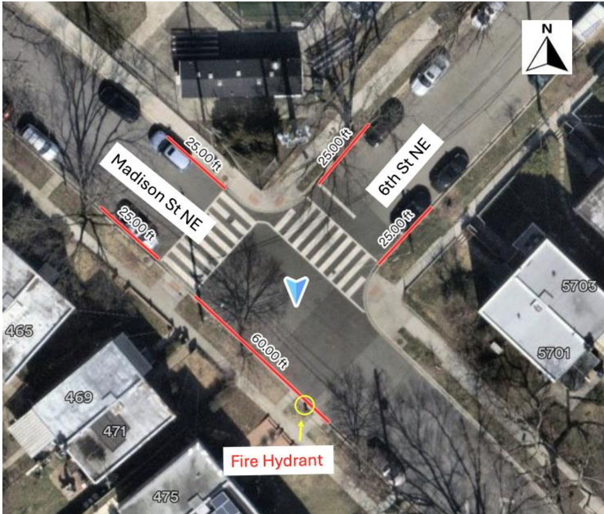
Figure 1: Proposed changes at the intersection of 6th and Madison NE. Each red line indicates length of each daylighting zone. White pavement markings and flexposts will be installed.
